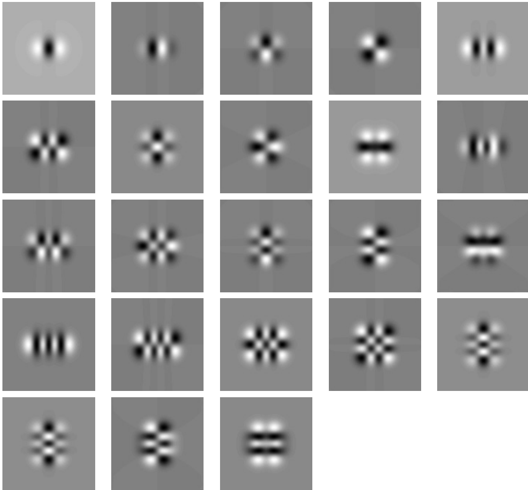
Figure 8: Orthogonal basis functions that steer (4x^2 - 2) \exp[-(x^2 + y^2)] under x, y -translation and rotation. The image at the top left is the function that was used as input to the procedure.
