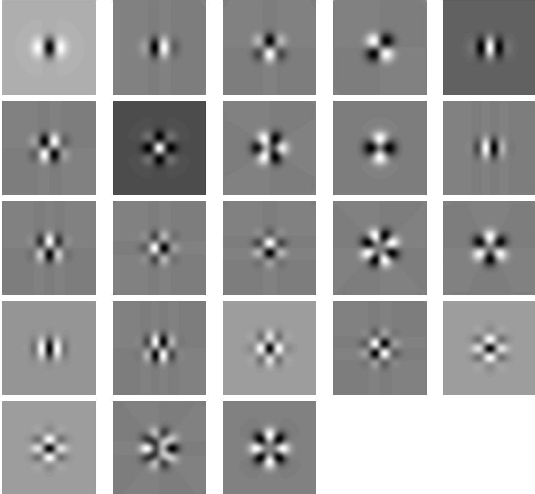
Figure 7: Basis functions that steer (4x^2 - 2) \exp[-(x^2 + y^2)] under x, y - translation and rotation. The image at the top left is the function that was used as input to the procedure.
