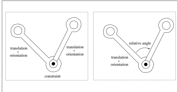
Fig. 2. Two possibilities of parameter sets for the pose definition of an articulated object having a revolute joint.
