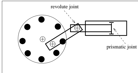
Fig. 1. An articulated object composed of rigid components connected by two revolute joints and a single prismatic joint.
