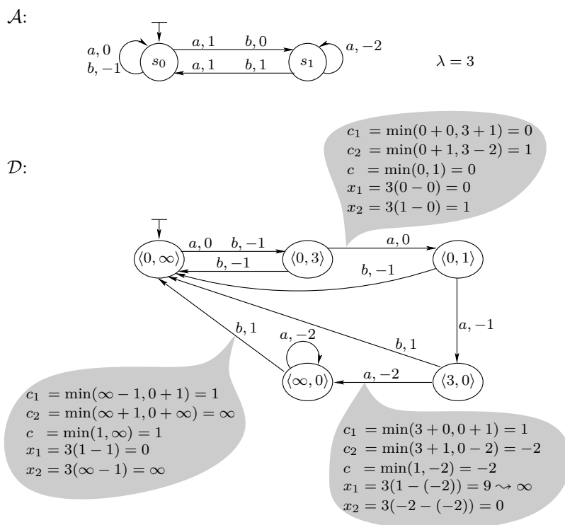
■ Figure 1 Determinizing the 3-NDA \mathcal{A} into the 3-DDA \mathcal{D} . The gray bubbles detail some of the intermediate calculations of the determinization procedure.
