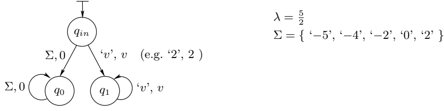
■ Figure 4 The non-determinizable \frac{5}{2} -NDA \mathcal{A} .
